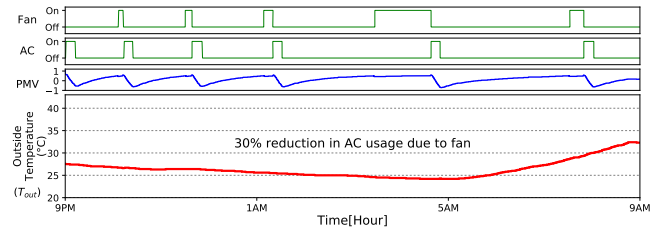
(b) PMV with fan (May 4th/5th)
