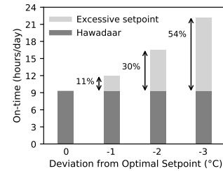
Figure 9: Optimal vs excessive: The standards-compliant HAWADAAR saves energy by prohibiting excessive setpoints.
