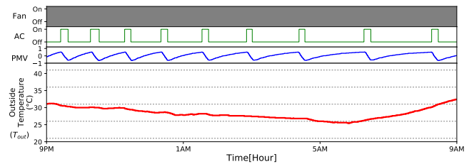
(a) PMV without fan (May 2nd/3rd)
