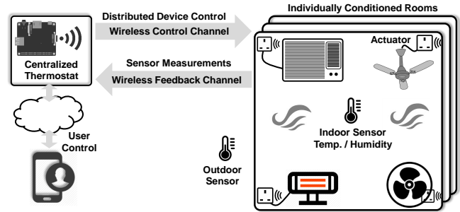
Figure 2: Inverted HVAC architecture: IoT retrofitting for distributed conditioning via a centralized control abstraction, to improve thermal comfort and energy efficiency of legacy buildings.
