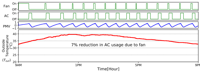
(b) PMV with fan (May 3rd)
